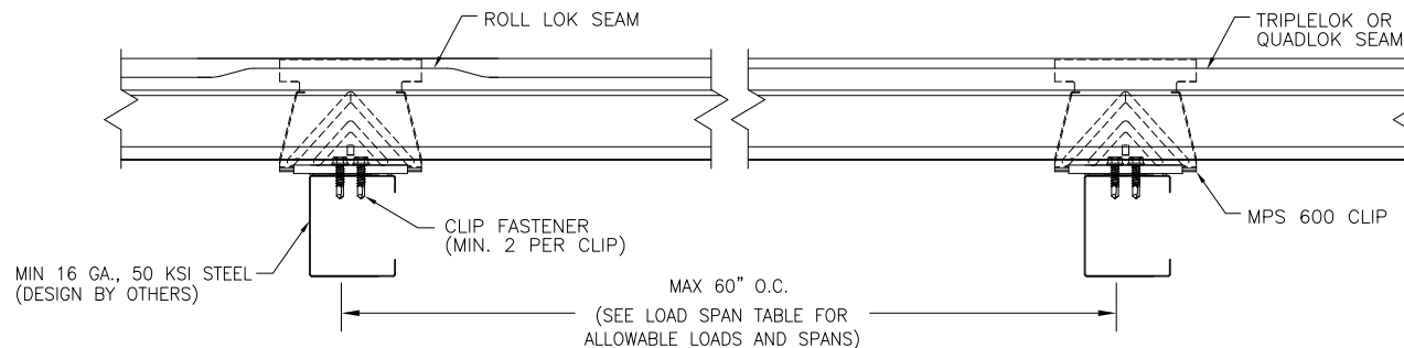
TYPICAL SIDE VIEW
