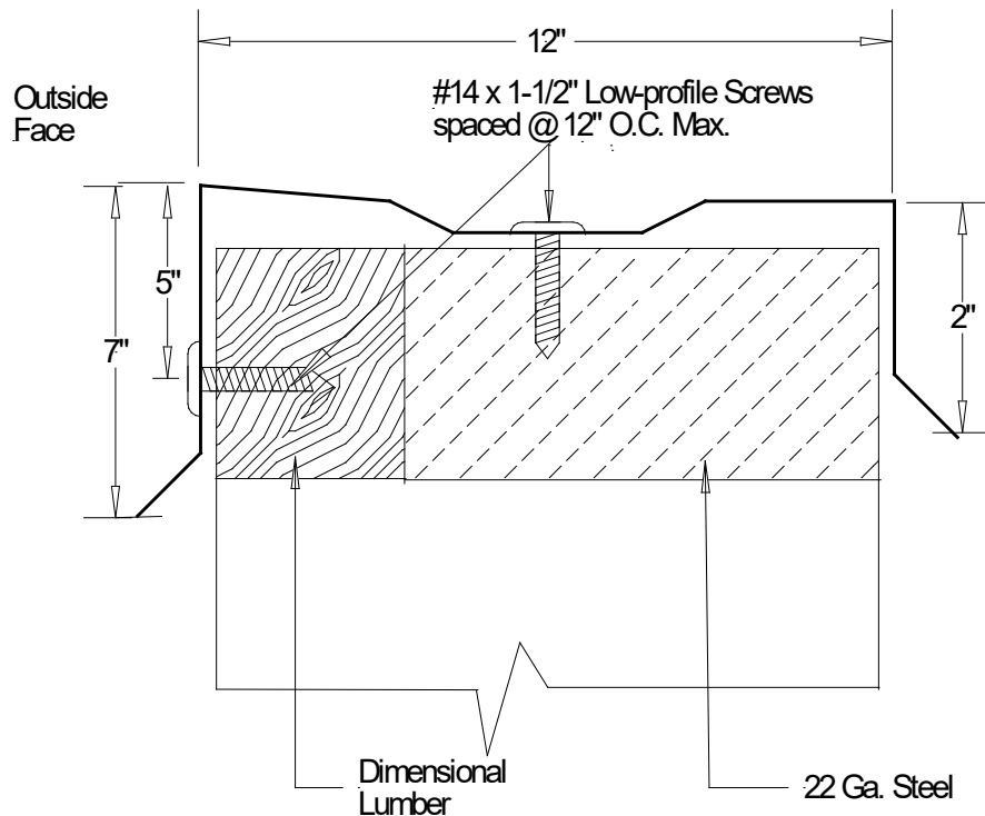
Typical Assembly Profile View
