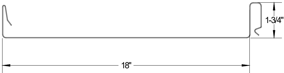
Typical Panel Profile View
