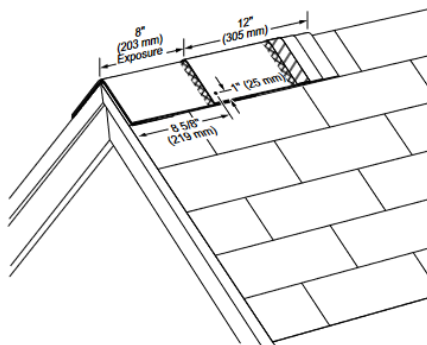
Figure 11-21: Install cap shingles at an 8 inch exposure and fasten with one nail on each side as shown.
