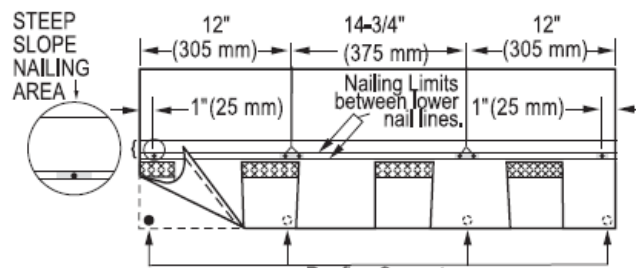
Four (4) Nail Attachment (2:12 to 21:12)
