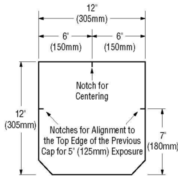
English Dimension
