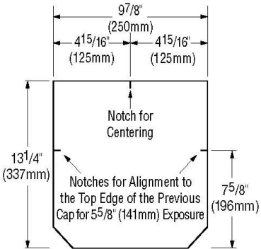
Metric Dimension
