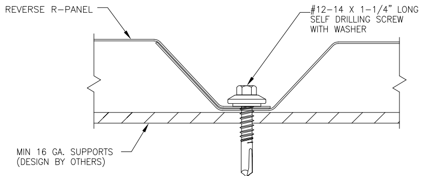
PANEL SIDELAP
