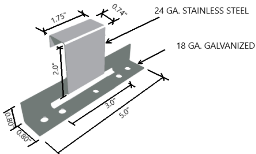
Panel Clip Profile "Expansion Clip" (2 Piece Sliding Clip)
