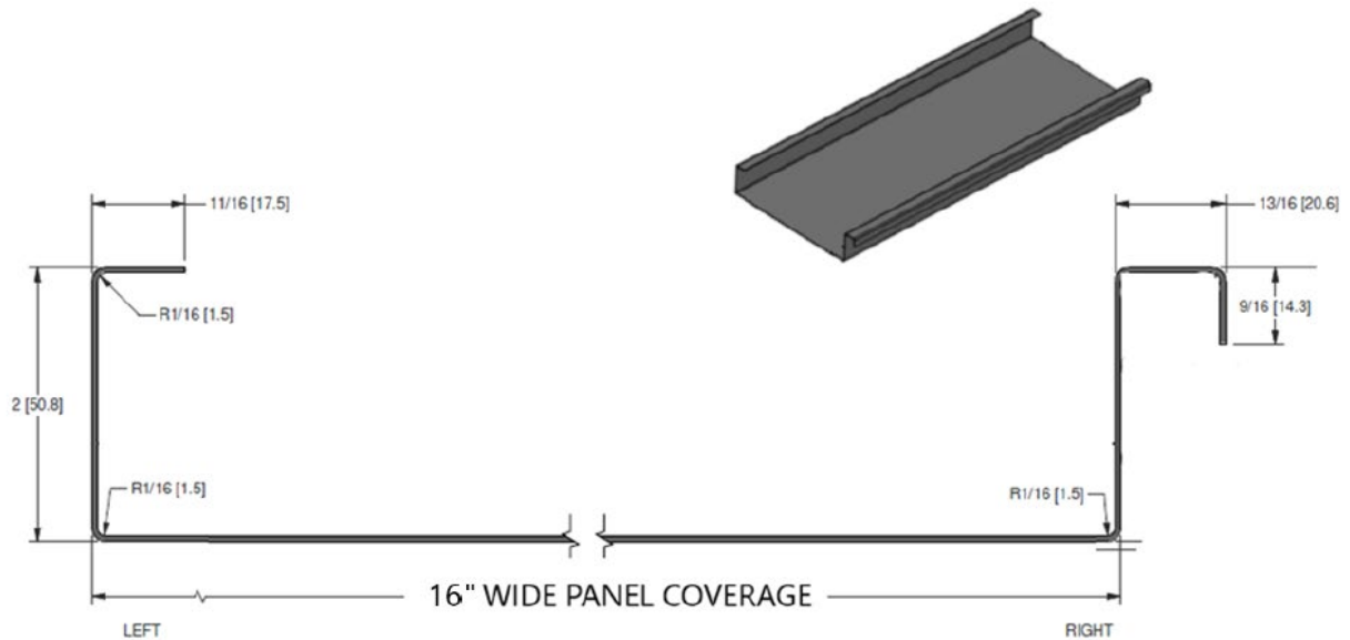
Typical Panel Profile
