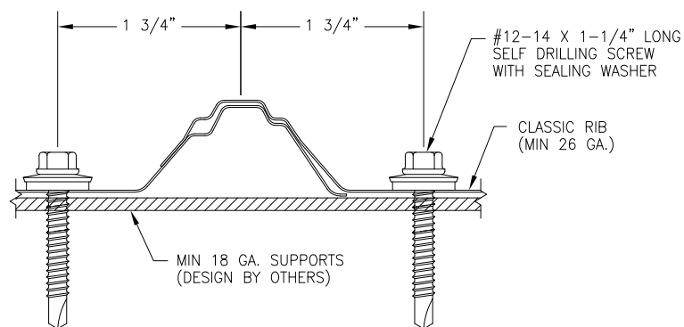
DETAIL 1
