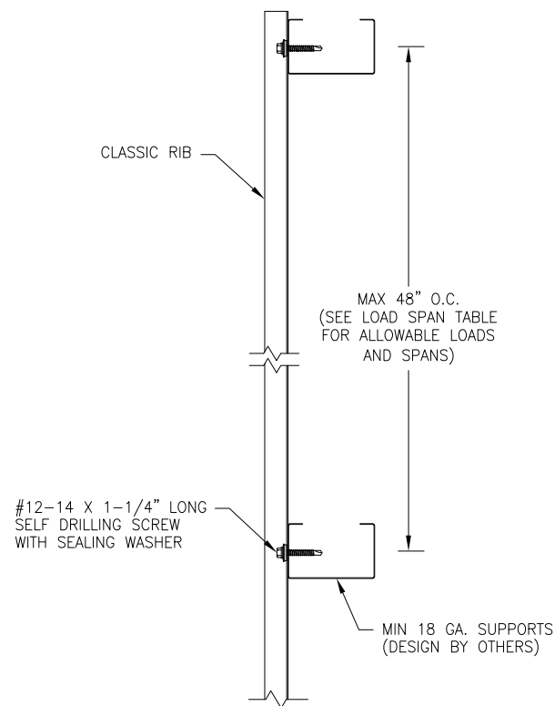
SECTION VIEW
