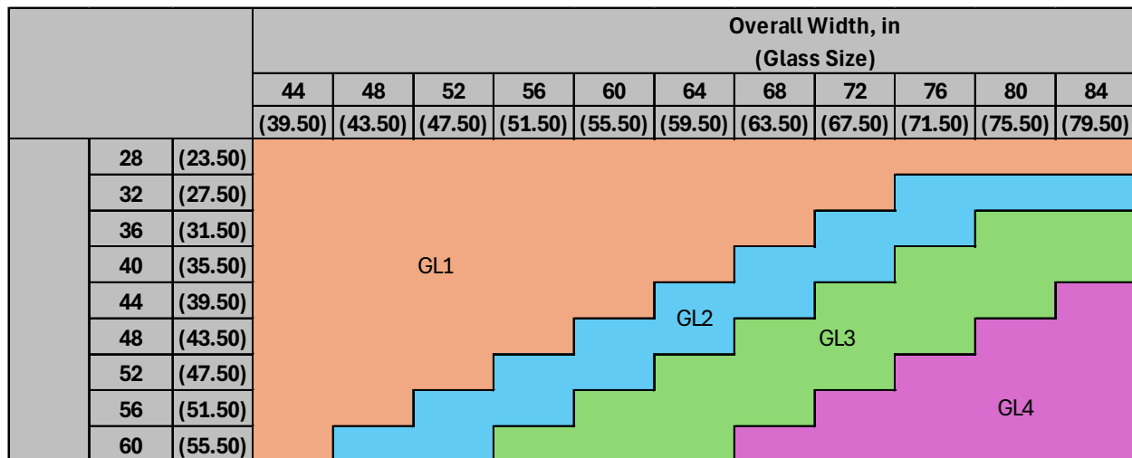
Chart 1: ASTM E1300 Glazing Requirements per Unit Size
