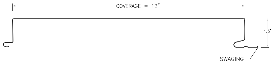
FW-120 PANEL PROFILE
