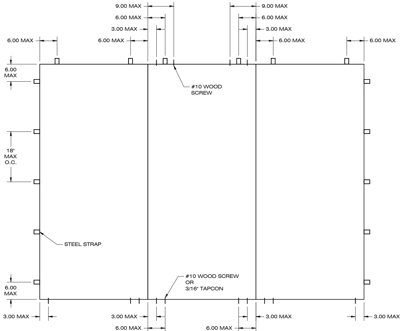
Single door with sidelites OXO
