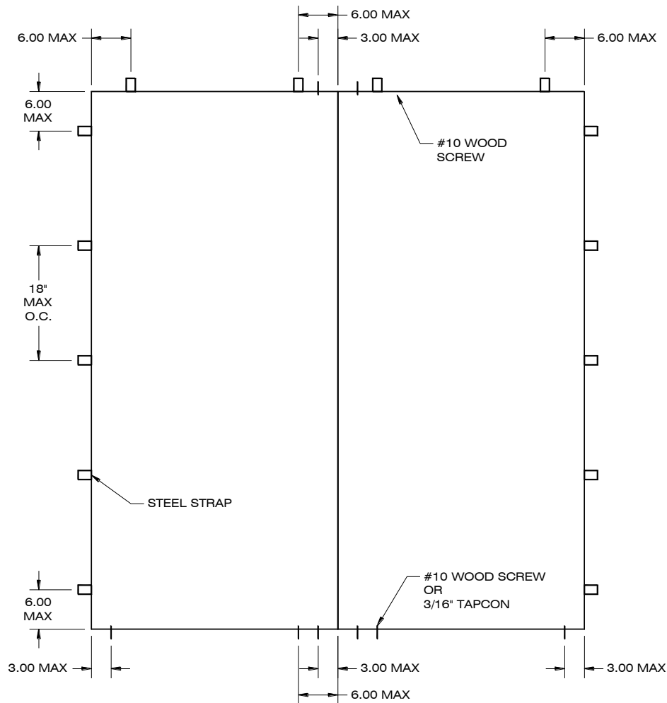
Single with sidelite OX or XO
