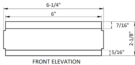
FLOATING TOP (PART No. 05082H)
