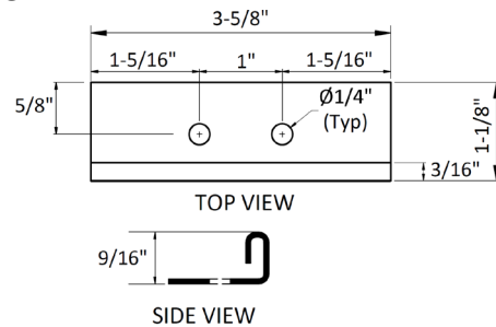
FLOATING BASE (PART No. 05082I)
