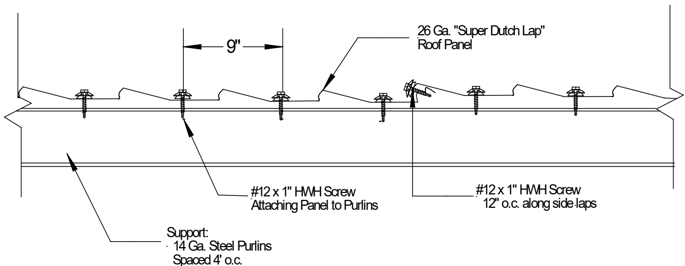
Roof Assembly Profile Typical Fastening Pattern along Supports
