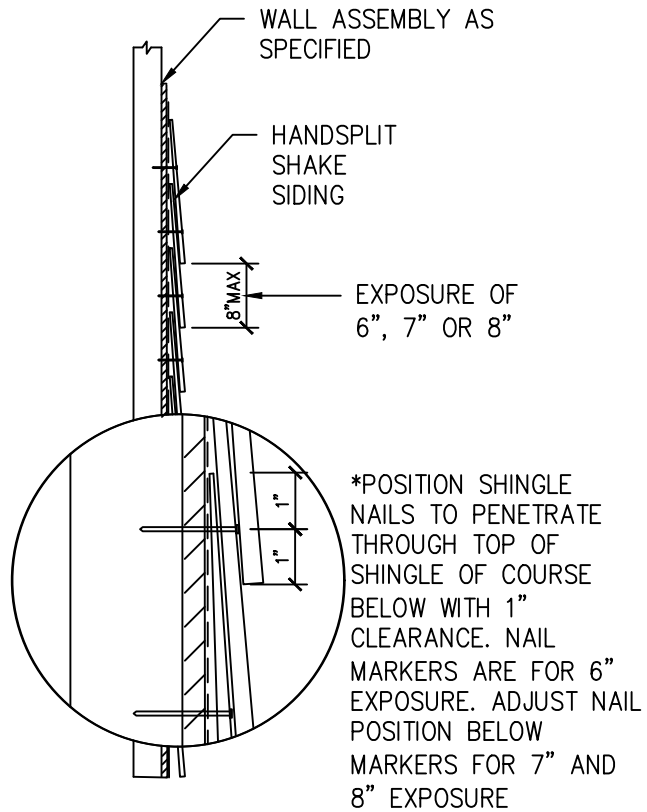
A 2 SIDING INSTALLATION SECTION VIEW NOT-TO-SCALE
