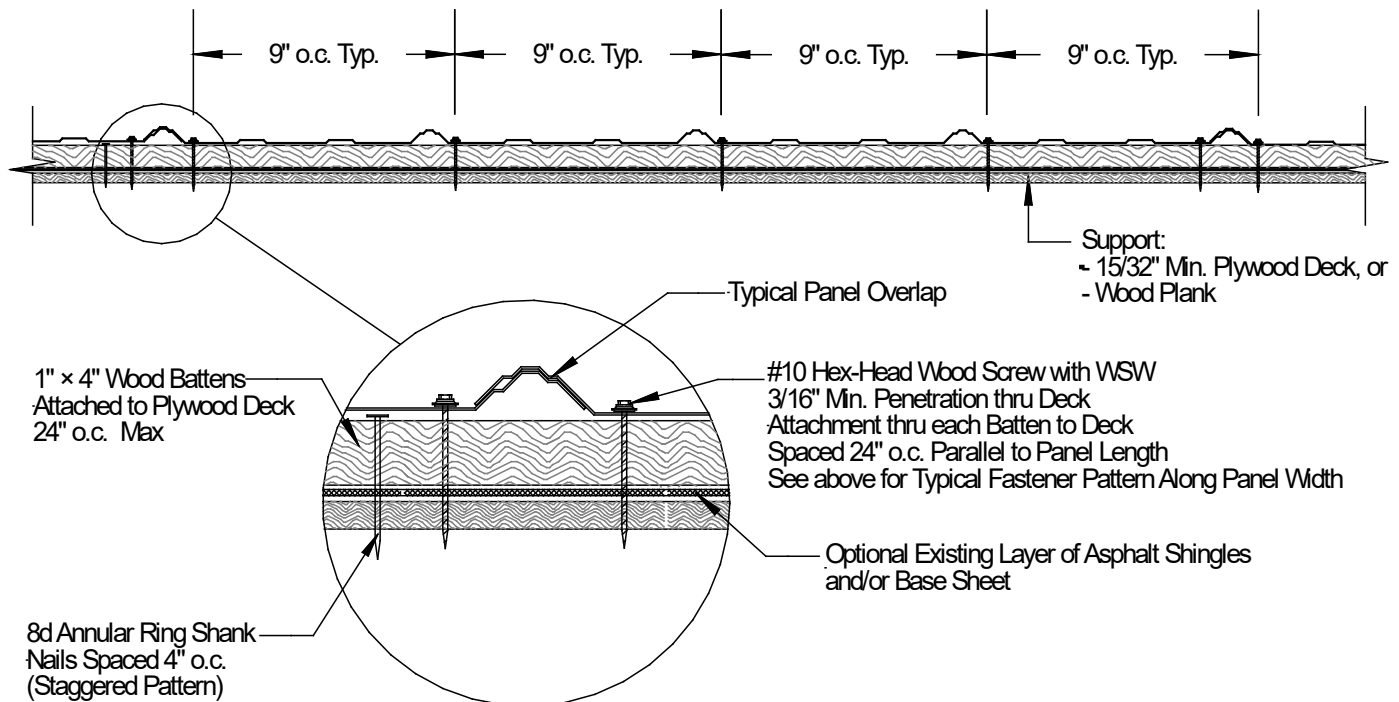
Typical Field of Panel Assembly Section View (N.T.S.)
