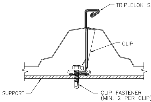
CLIP SECTION VIEW DETAIL 1
