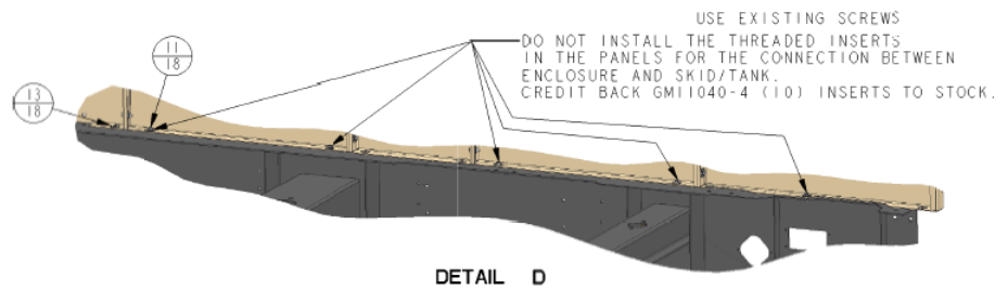
DETAIL D
