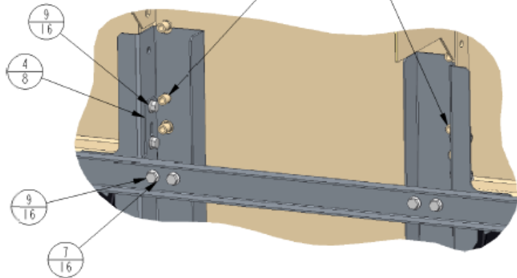
DETAIL B
