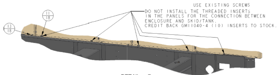
DETAIL D
