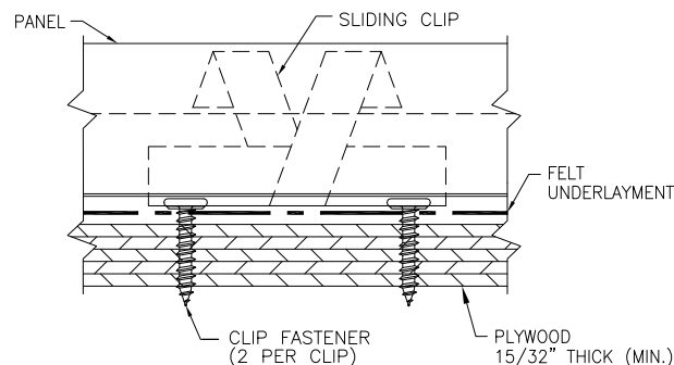
DETAIL 1
