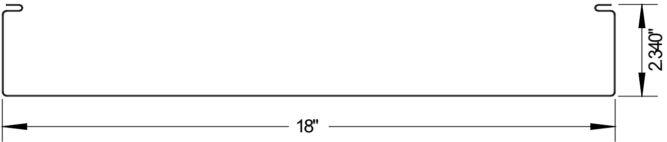
Berridge Tee-Lock Typical Panel Profile
