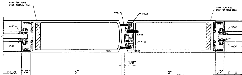
4 MEETING STILE S/A
