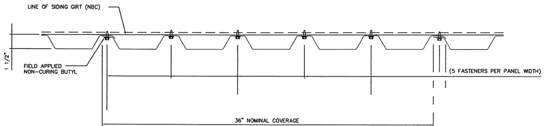
FASTENING SCHEDULE (LEFT TO RIGHT ERECTION)
