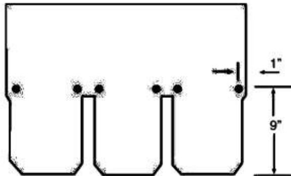
Figure 10. StormMaster® Slate 6 Nail Pattern
