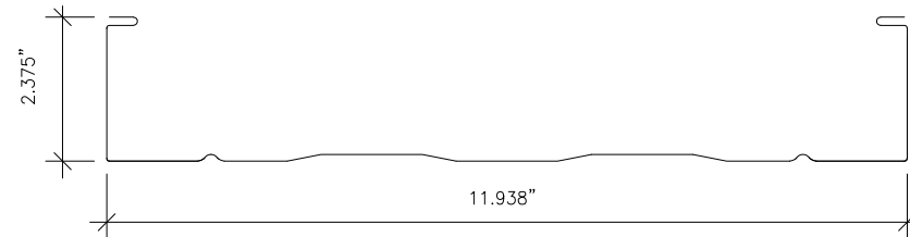
PANEL SECTION (MIN 0.04" THICK ALUMINUM)
