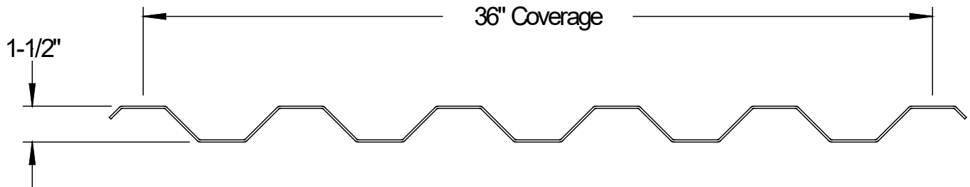
Typical Panel Profile
