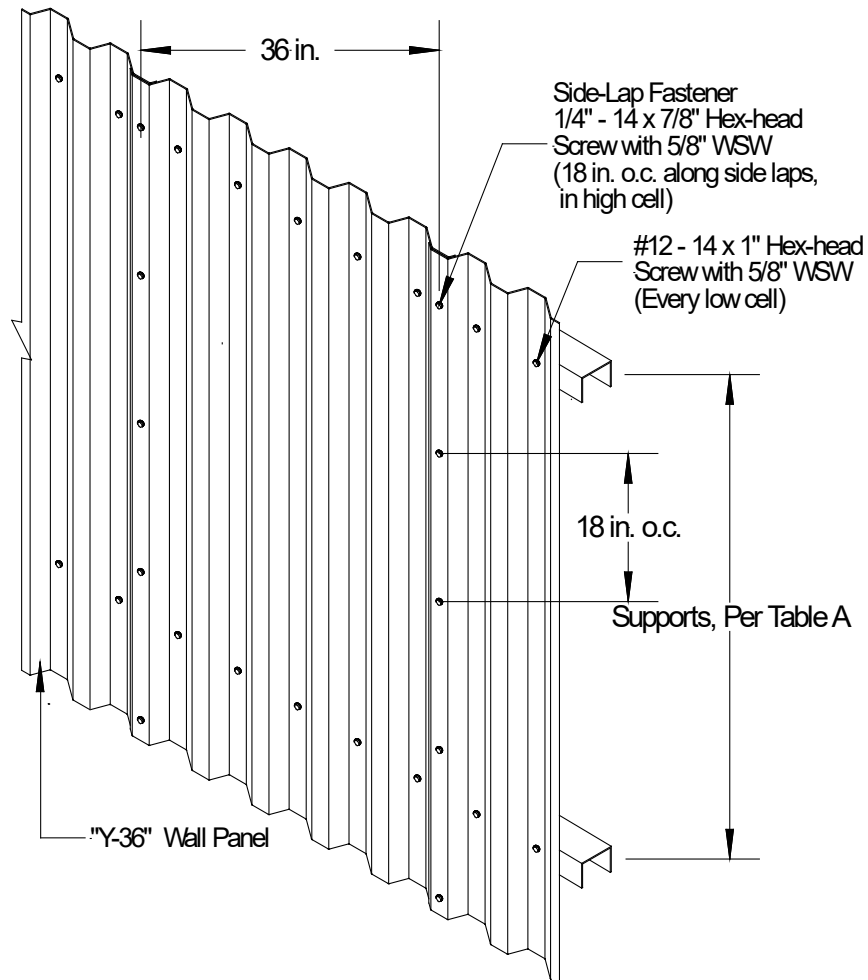
"Vertical Series" Typical Assembly Isometric View
