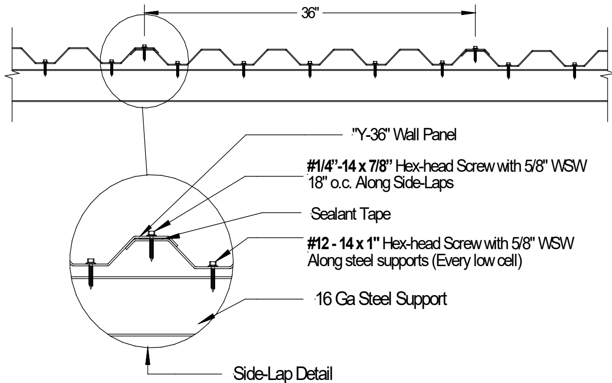
Assembly Profile View Typical Fastening Pattern Across Row
