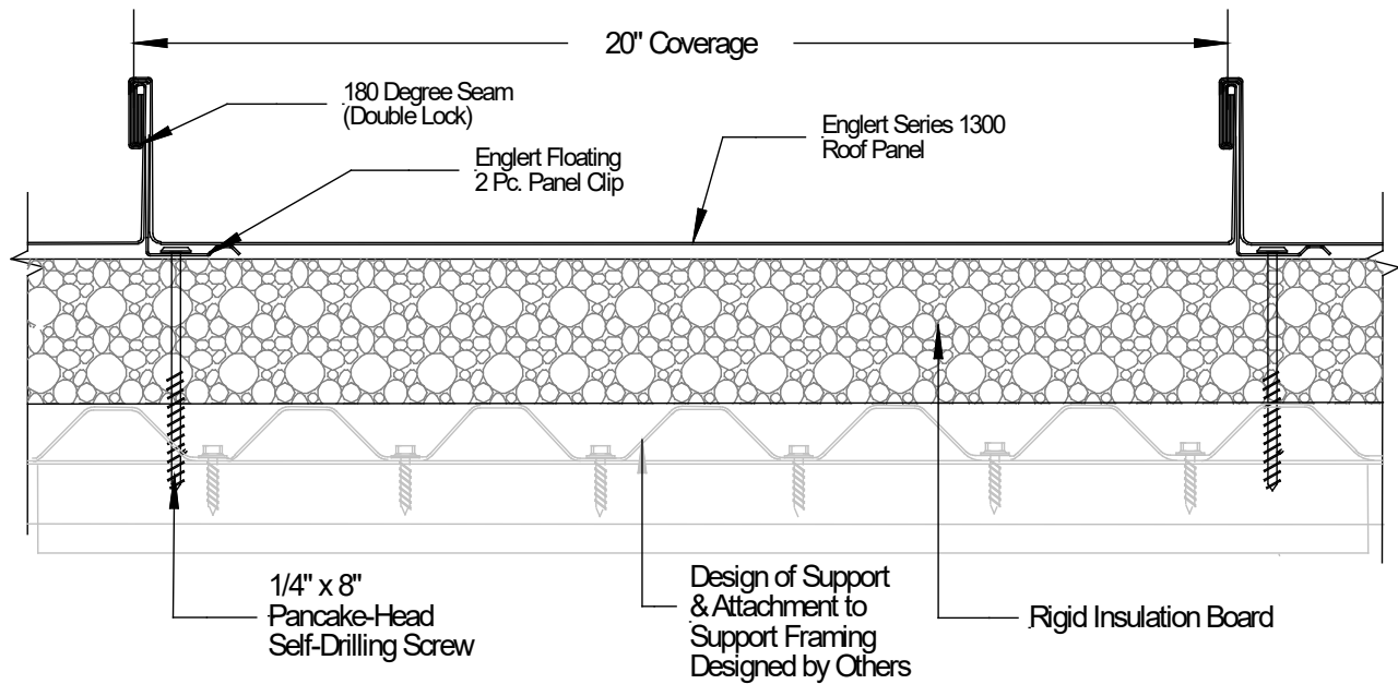
Typical Assembly Profile View (Typical Fastening Pattern Across Width)
