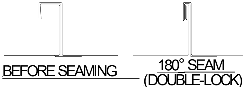
Typical Panel Seam
