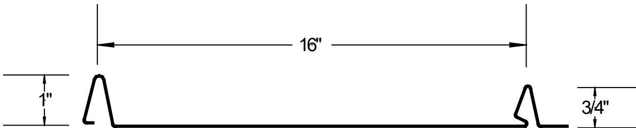
Panel Profile
