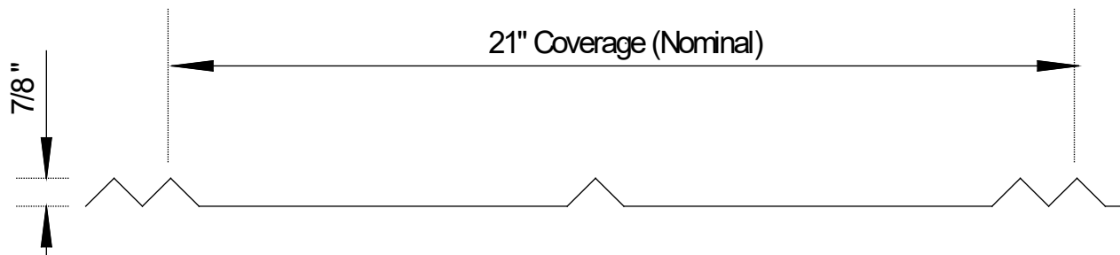
Panel Profile
