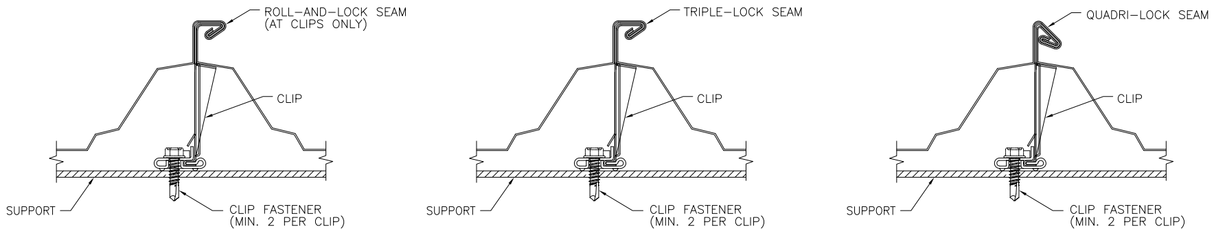
CLIP SECTION VIEW DETAIL 1
