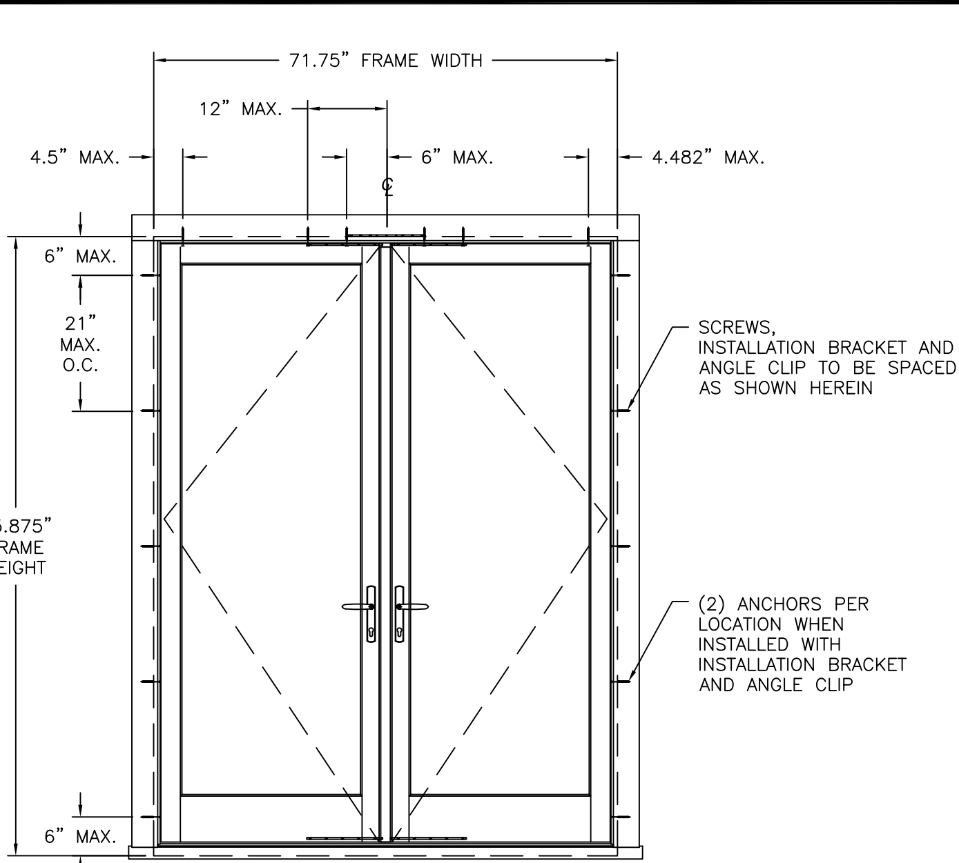
FRENCH IS WOOD DOUBLE DOOR EXTERIOR VIEW ANCHORS THROUGH FRAME
