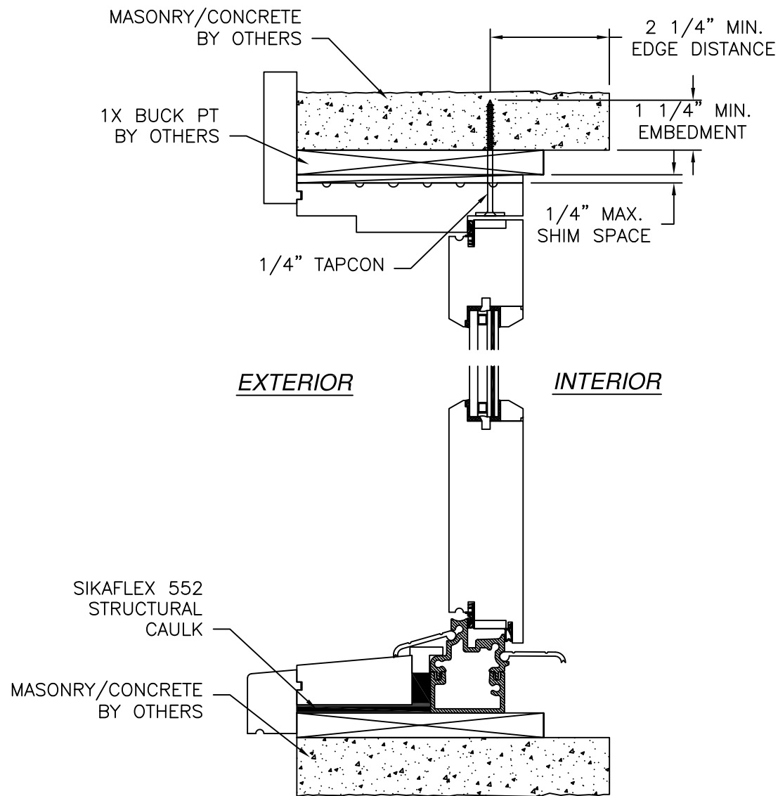
VERTICAL CROSS SECTION CONCRETE/MASONRY INSTALLATION
