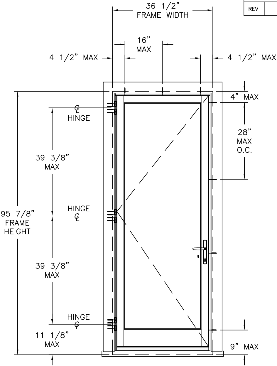
FRENCH IS WOOD SINGLE DOOR EXTERIOR VIEW ANCHORS THROUGH HARDWARE & HINGES
