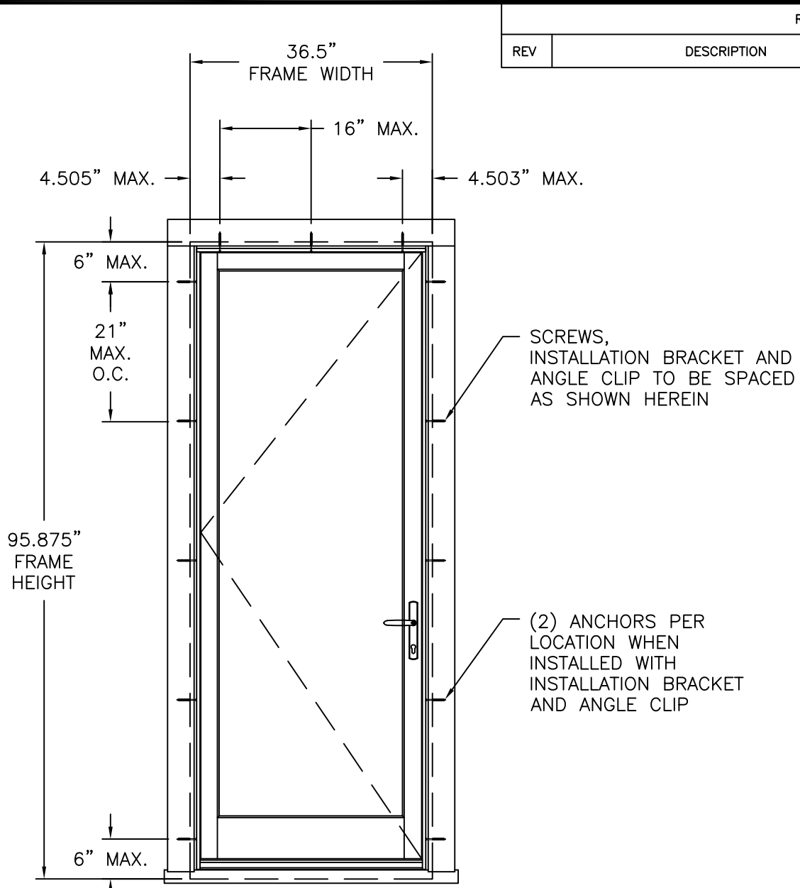
FRENCH IS WOOD SINGLE DOOR EXTERIOR VIEW ANCHORS THROUGH FRAME
