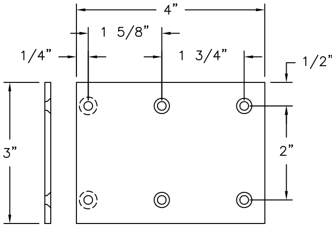
ALUMINUM 6063-T5 .125 " THICK
