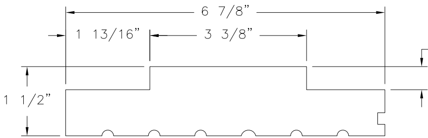
JAMB MAHOGANY
