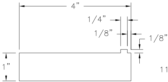
CASING MAHOGANY
