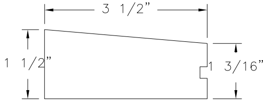
DOOR SILL MAHOGANY
