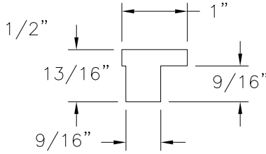
SUPPORT BLOCK MAHOGANY
