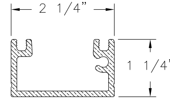
SILL EXTRUSION BRONZE
