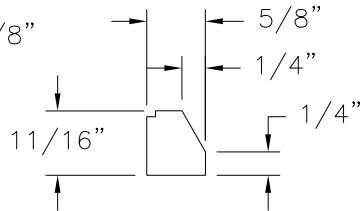
GLAS STOP MAHOGANY
