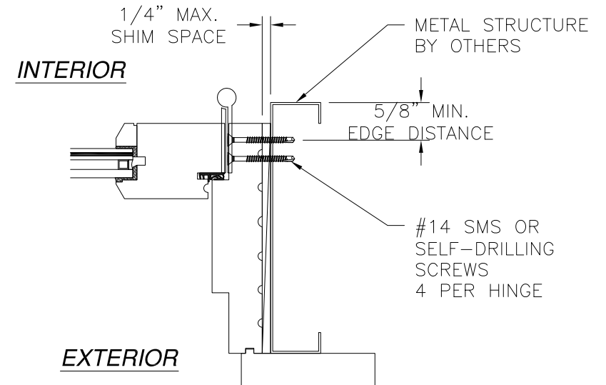
JAMB INSTALLATION DETAIL THROUGH HINGE INSTALLATION INTO METAL STRUCTURE
