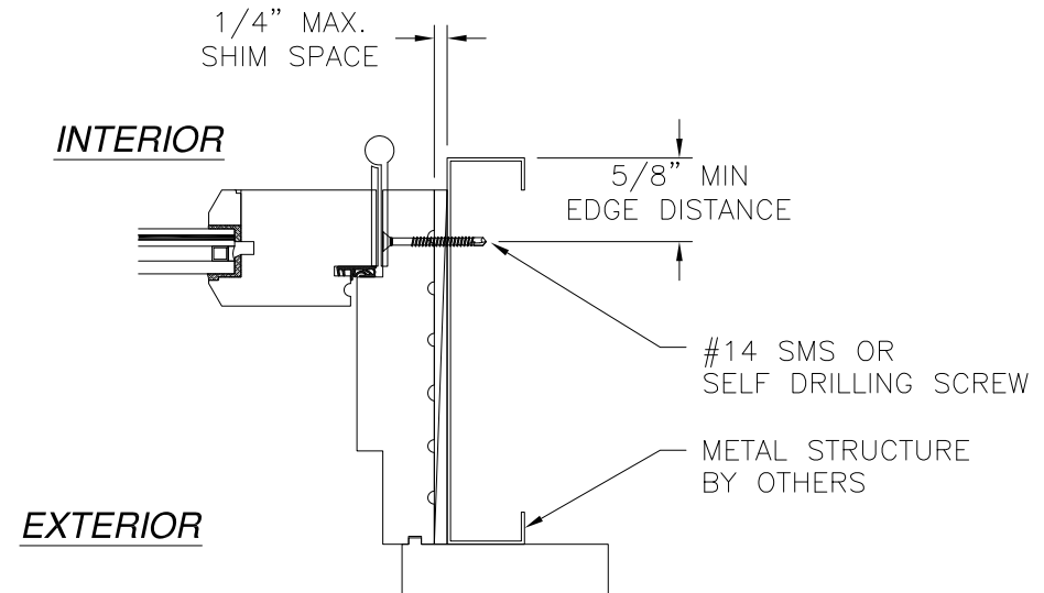
JAMB INSTALLATION DETAIL THROUGH FRAME INSTALLATION INTO METAL STRUCTURE
