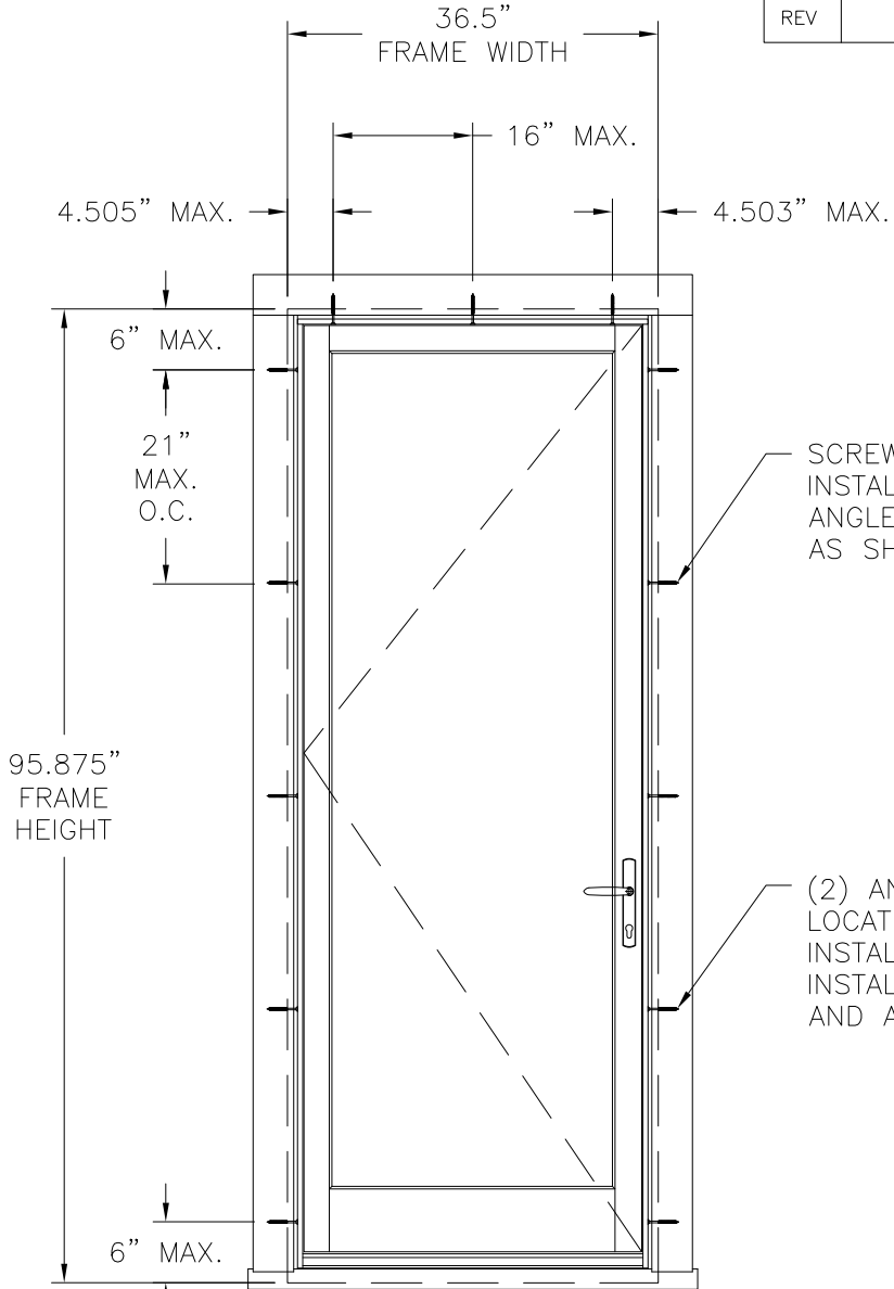
FRENCH IS WOOD SINGLE DOOR EXTERIOR VIEW ANCHORS THROUGH FRAME
