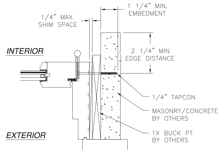
JAMB INSTALLATION DETAIL THROUGH FRAME INSTALLATION INTO MASONRY/CONCRETE
