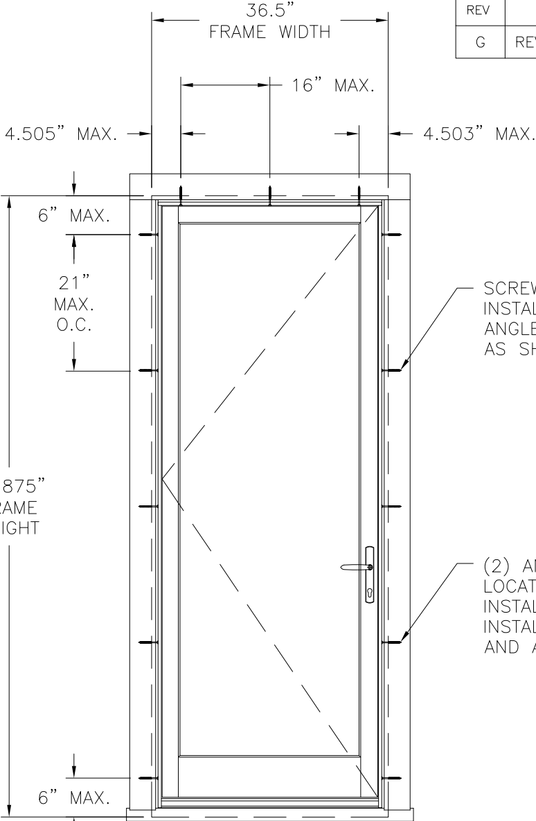
FRENCH IS WOOD SINGLE DOOR EXTERIOR VIEW ANCHORS THROUGH FRAME
