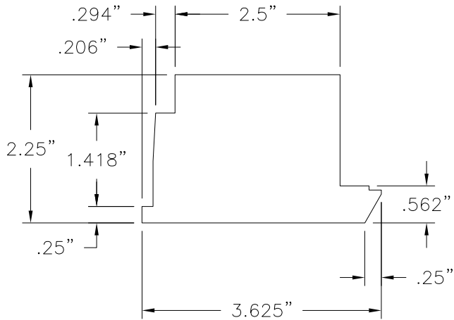
② STILE/RAIL MAHOGANY
