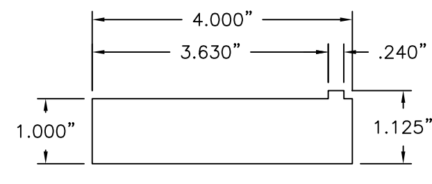
⑦ CASING MAHOGANY
