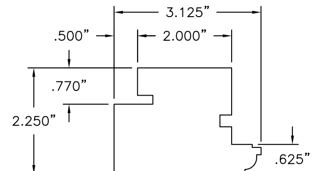
⑤ HEAD RAIL/STILE MAHOGANY
