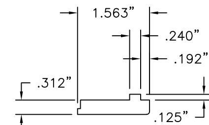
⑩ JAMB STOP MAHOGANY
