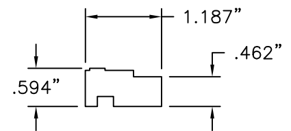
⑨ JAMB STOP MAHOGANY
