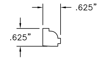
⑧ GLASS STOP MAHOGANY
