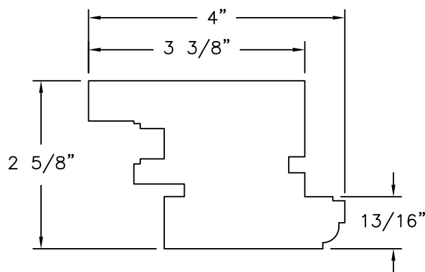
② STILE MAHOGANY
