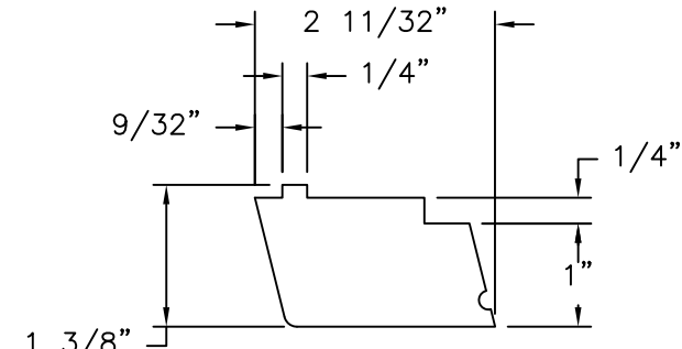
⑩ SILL NOSING MAHOGANY
