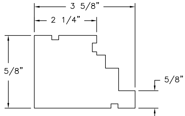
⑧ JAMB LEGS MAHOGANY
