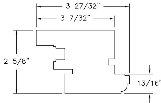
③ HEAD RAIL MAHOGANY
