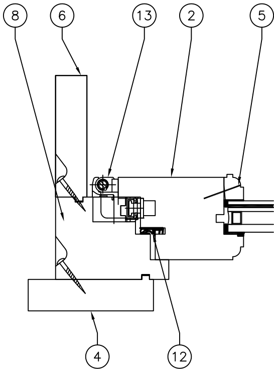
SECTION C-C
