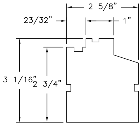
⑨ SILL MAHOGANY
