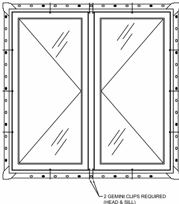
EXTERIOR ELEVATION
