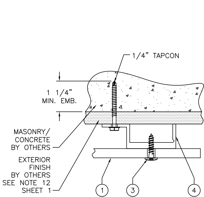
SECTION B-B INSTALLATION DETAIL MASONRY/CONCRETE
