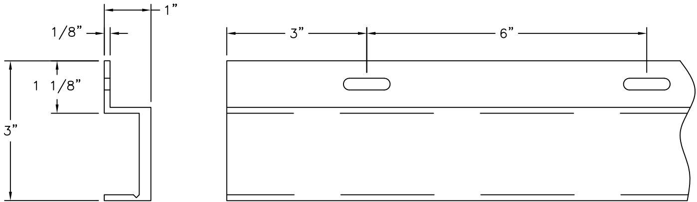
② J-CHANNEL ALUMINUM 6063-T6 .125" THICK 10' MAX. LENGTH
