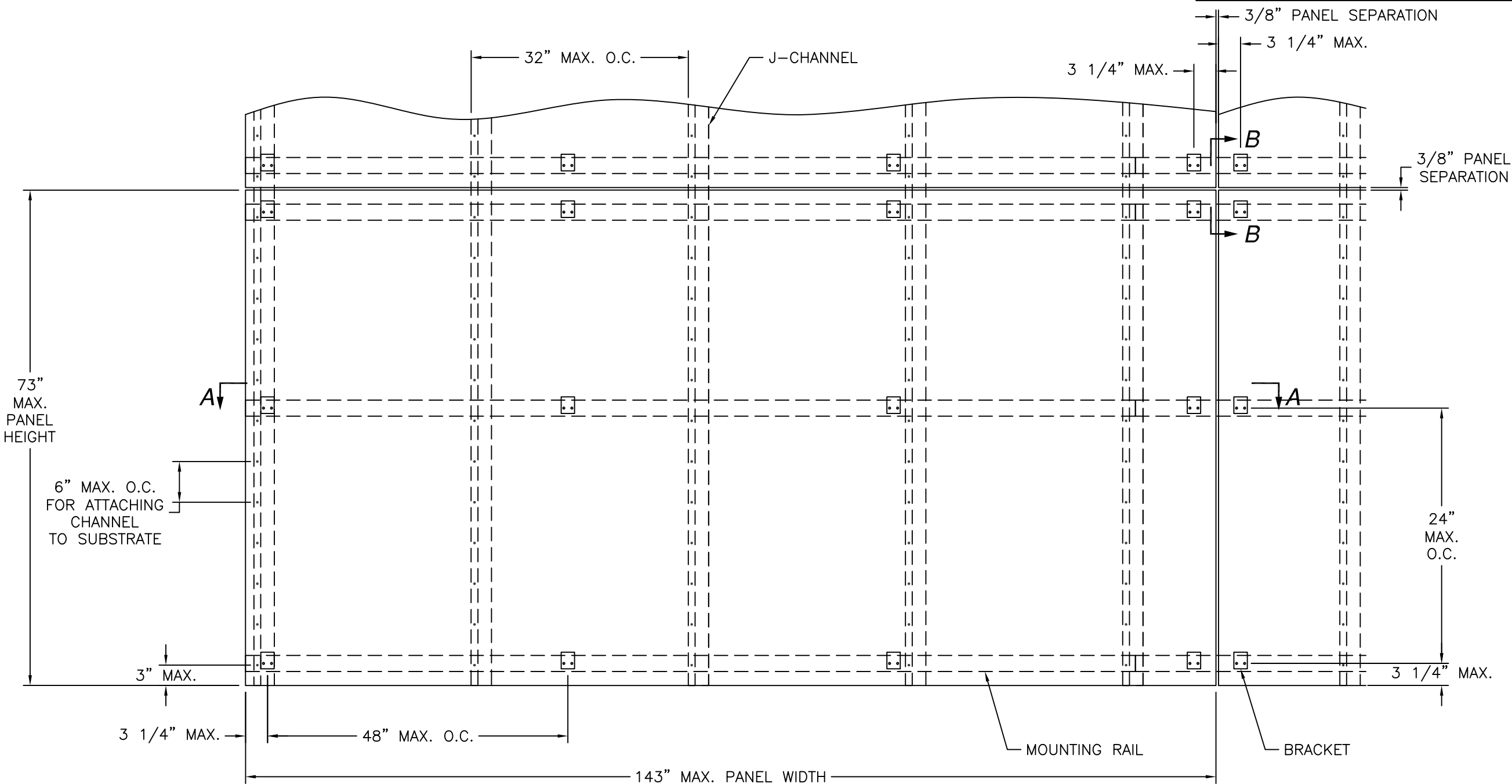
TYPICAL PANEL INSTALLATION ELEVATION
