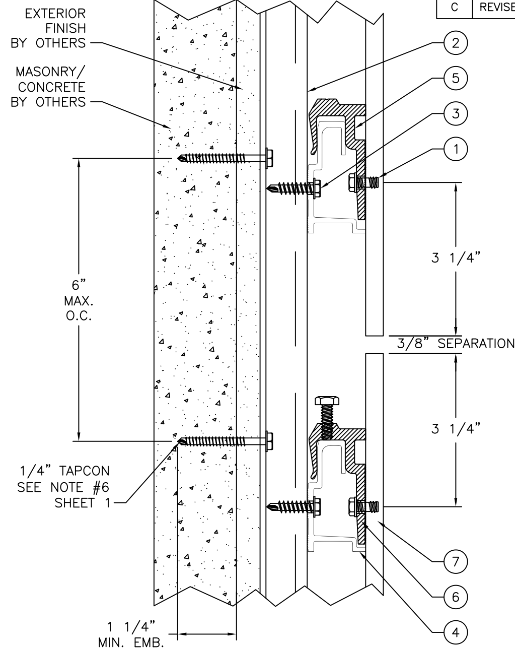
SECTION B-B INSTALLATION DETAIL MASONRY/CONCRETE
