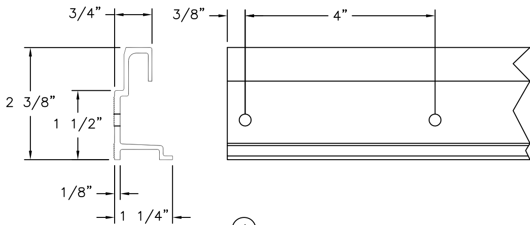
④ MOUNTING RAIL ALUMINUM 6063-T6 .125" THICK 12' MAX. LENGTH
