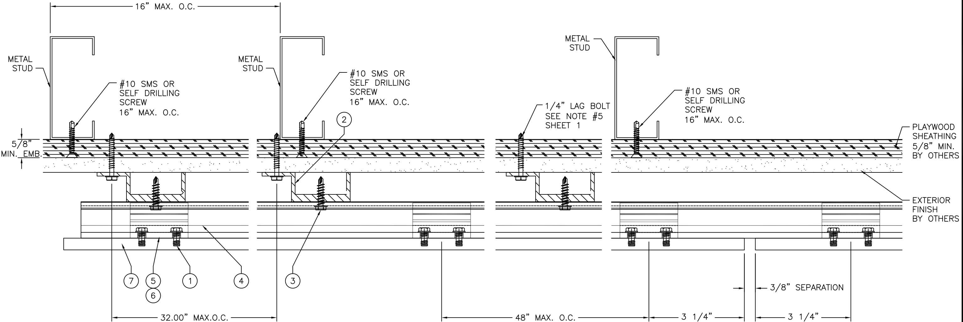
SECTION A-A INSTALLATION DETAIL 5/8" PLYWOOD SHEATHING (METAL FRAMING)
