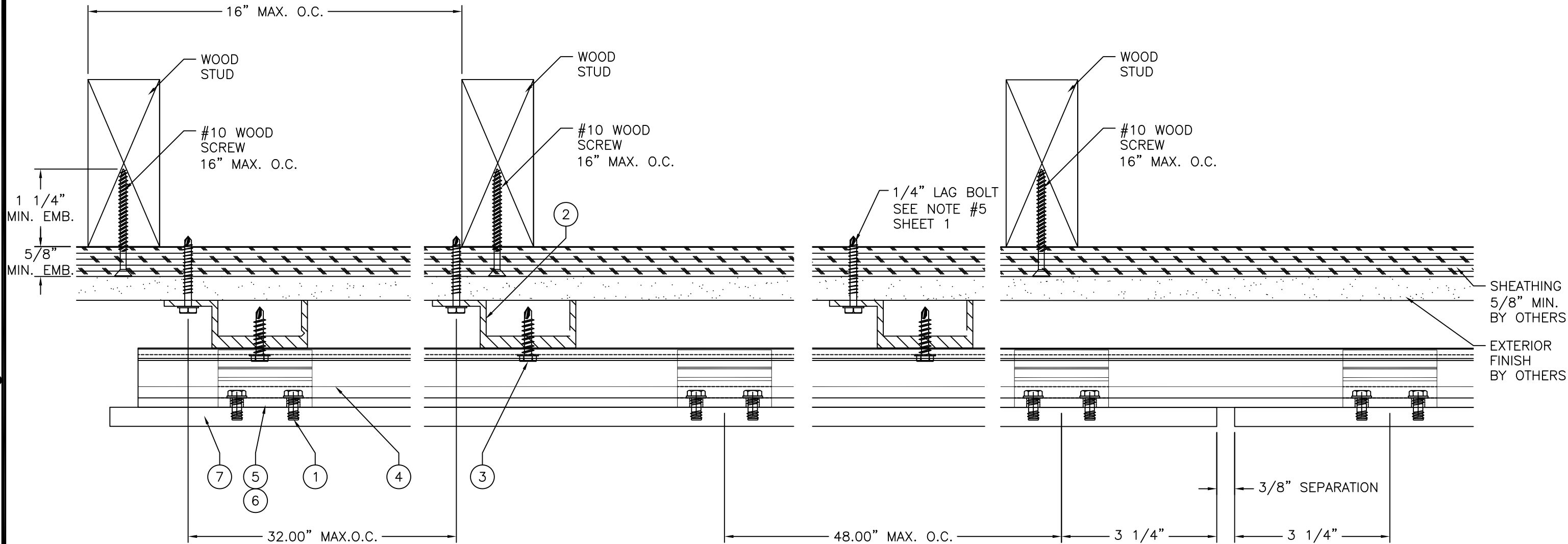
SECTION A-A INSTALLATION DETAIL 5/8" PLYWOOD SHEATHING (WOOD FRAMING)
