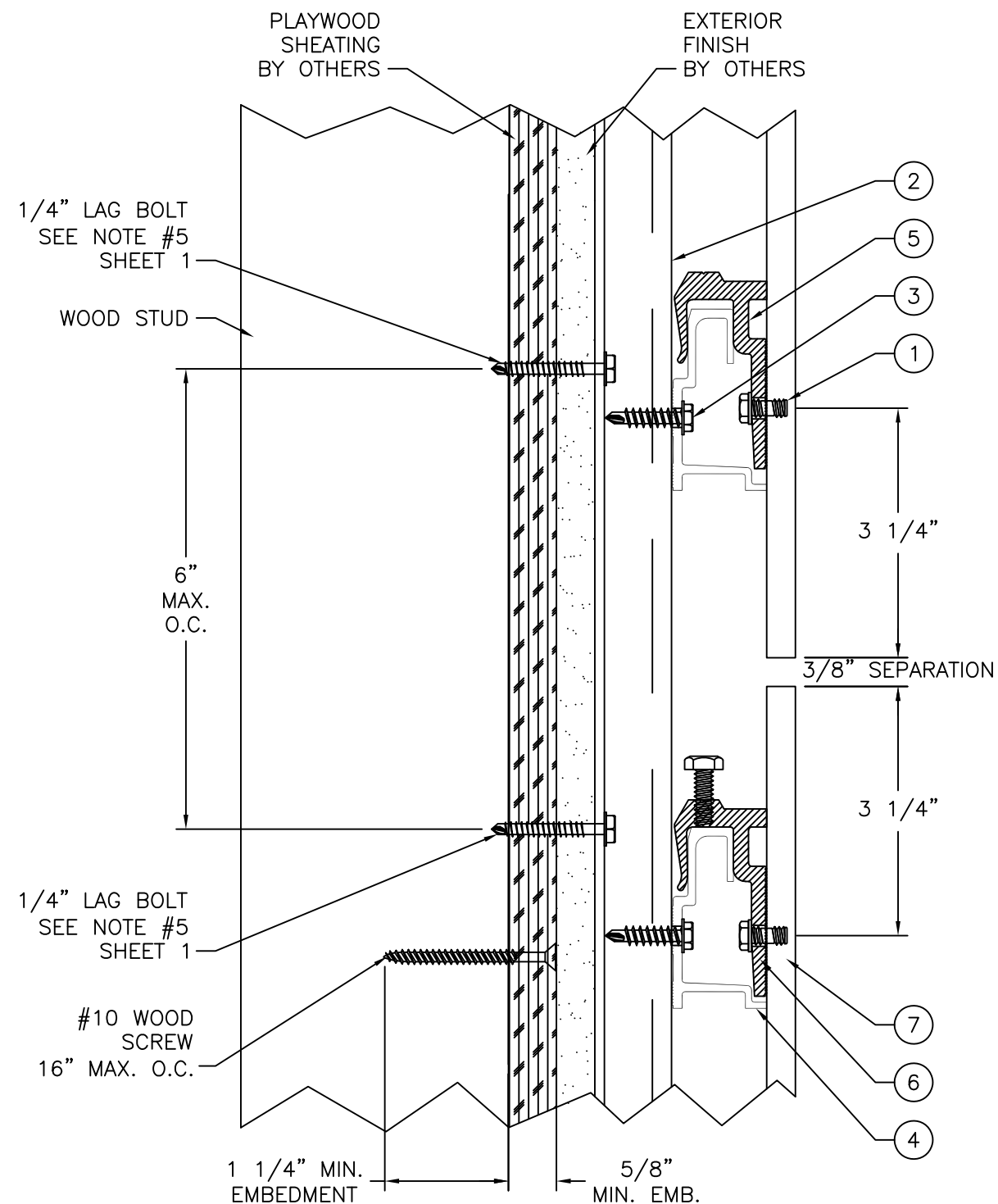
SECTION B-B INSTALLATION DETAIL 5/8" PLYWOOD SHEATHING (WOOD FRAMING)
