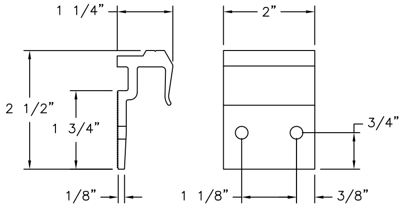
⑤ FIXED BRACKET ALUMINUM 6063-T6 .125" THICK
