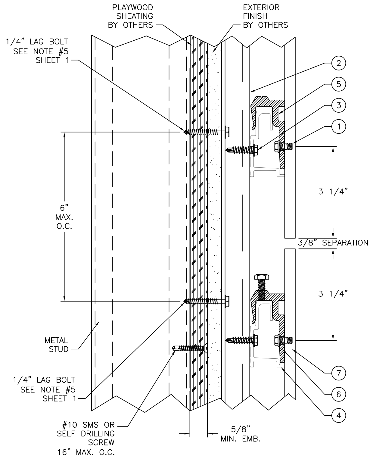
SECTION B-B INSTALLATION DETAIL 5/8" PLYWOOD SHEATHING (METAL FRAMING)
