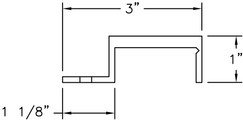
④ J-CHANNEL ALUMINUM 6063-T6 .125" THICK 10' MAX. LENGTH
