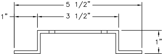
② HAT CHANNEL ALUMINUM 6063-T6 .125" THICK 10' MAX. LENGTH
