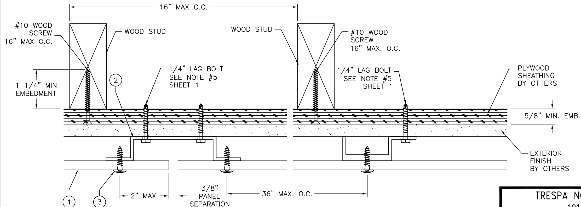
SECTION A-A INSTALLATION DETAIL 5/8" PLYWOOD SHEATHING INSTALLATION (WOOD FRAMING)
