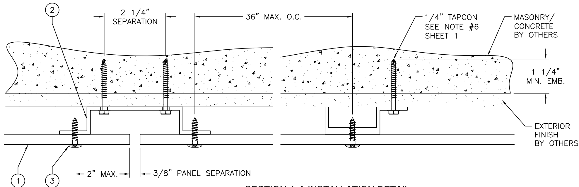
SECTION A-A INSTALLATION DETAIL MASONRY/CONCRETE
