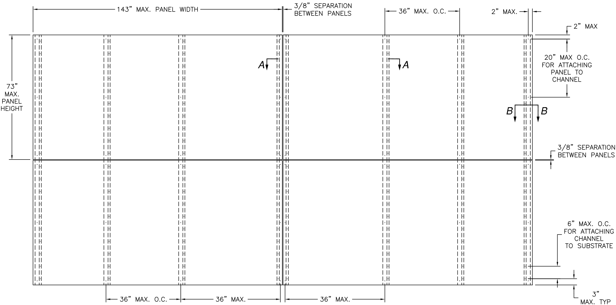
TYPICAL PANEL INSTALLATION ELEVATION
