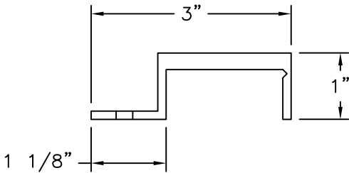
④ J-CHANNEL ALUMINUM 6063-T6 .125" THICK 10' MAX. LENGTH
