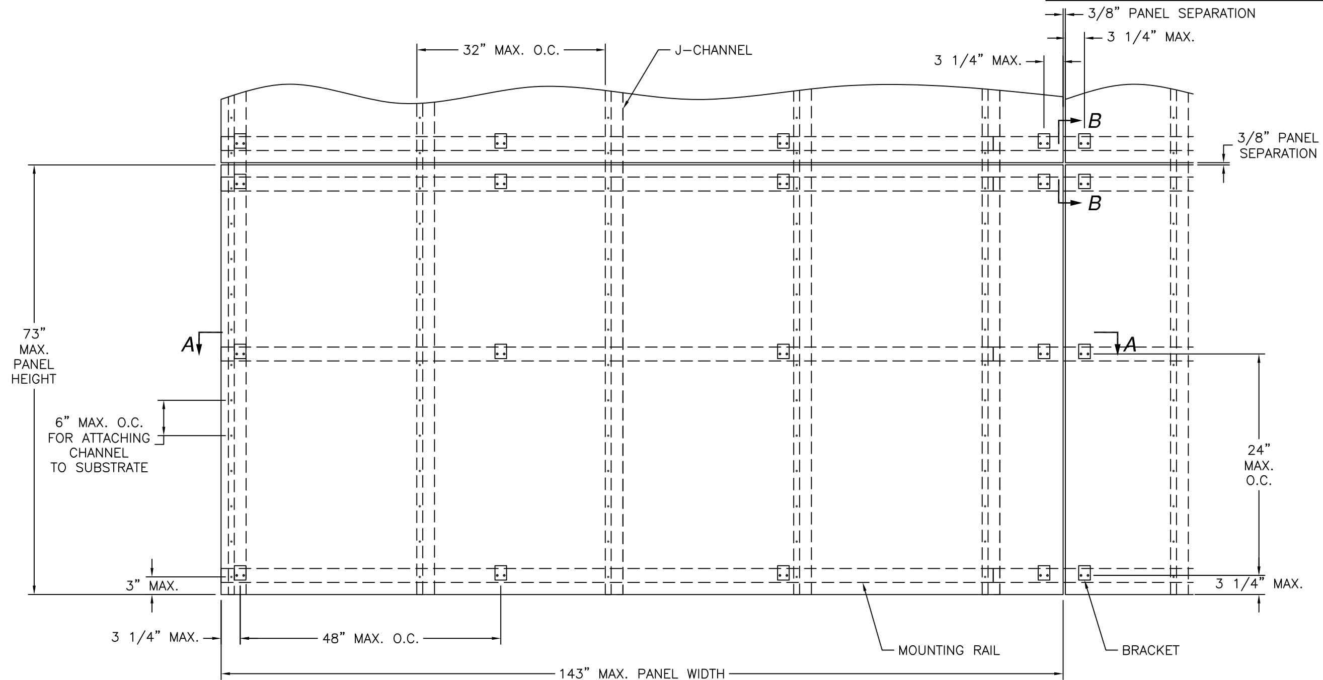
TYPICAL PANEL INSTALLATION ELEVATION
