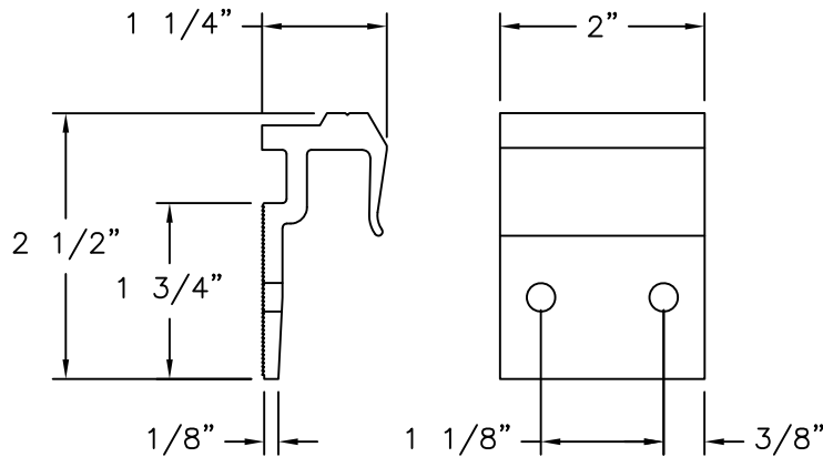
⑤ FIXED BRACKET ALUMINUM 6063-T6 .125" THICK
