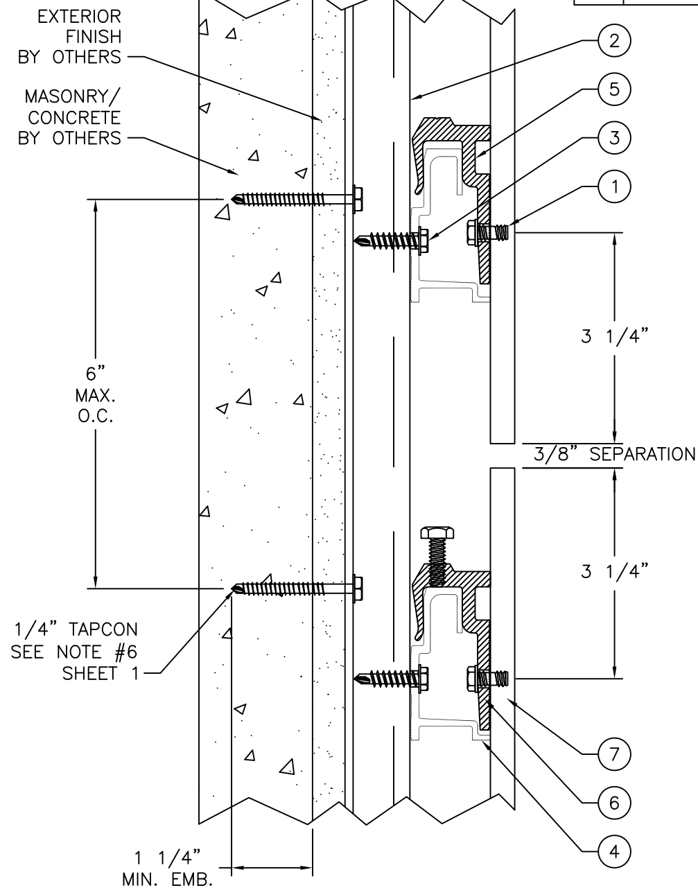
SECTION B-B INSTALLATION DETAIL MASONRY/CONCRETE
