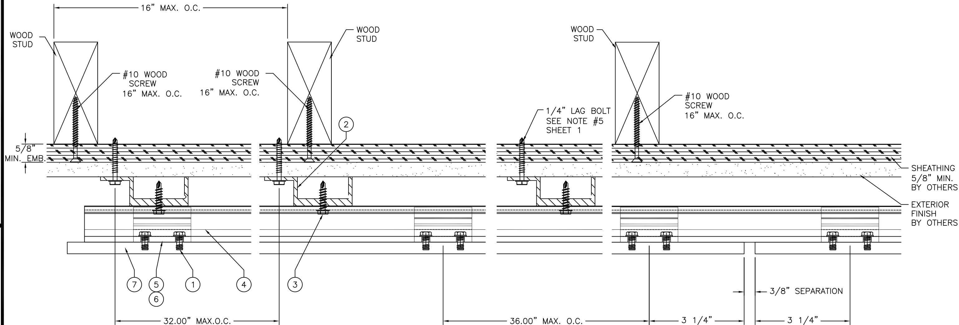
SECTION A-A INSTALLATION DETAIL 5/8" PLYWOOD SHEATHING (WOOD FRAMING)
