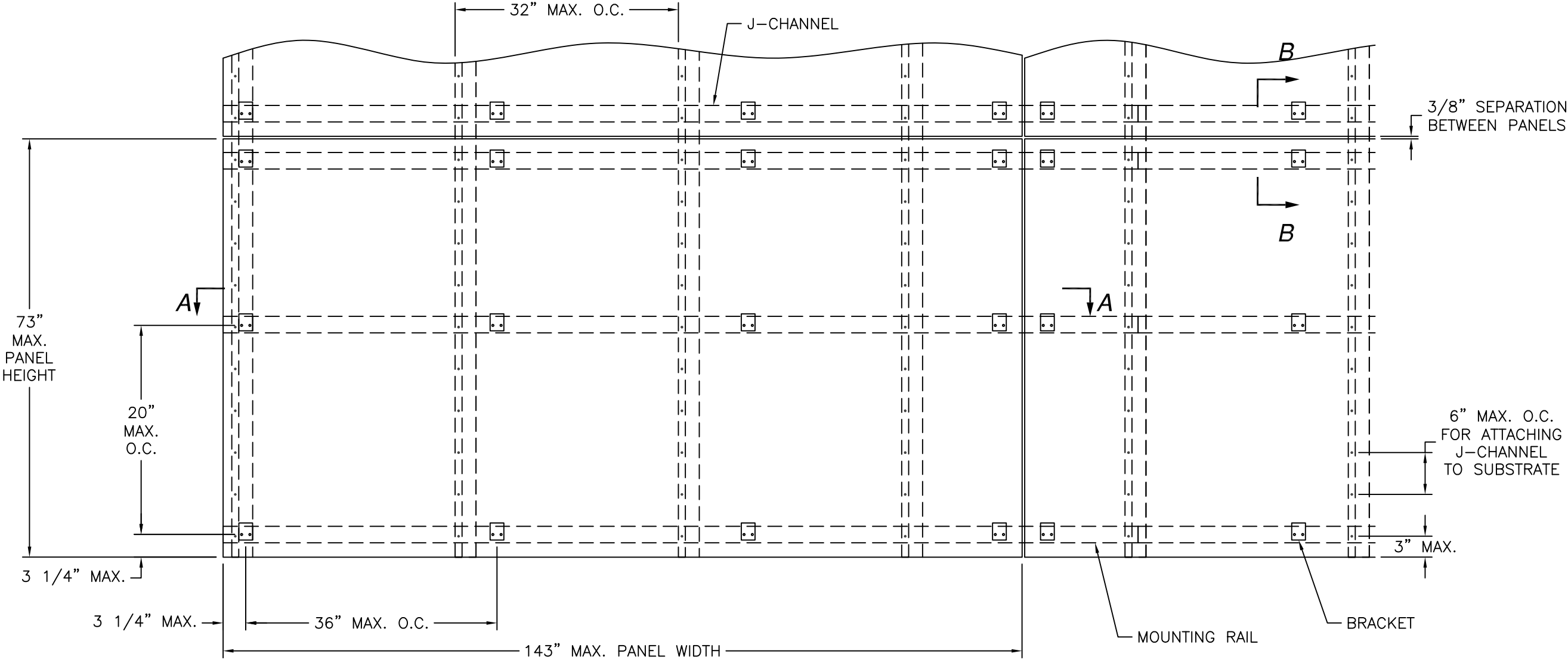
TYPICAL PANEL INSTALLATION ELEVATION
