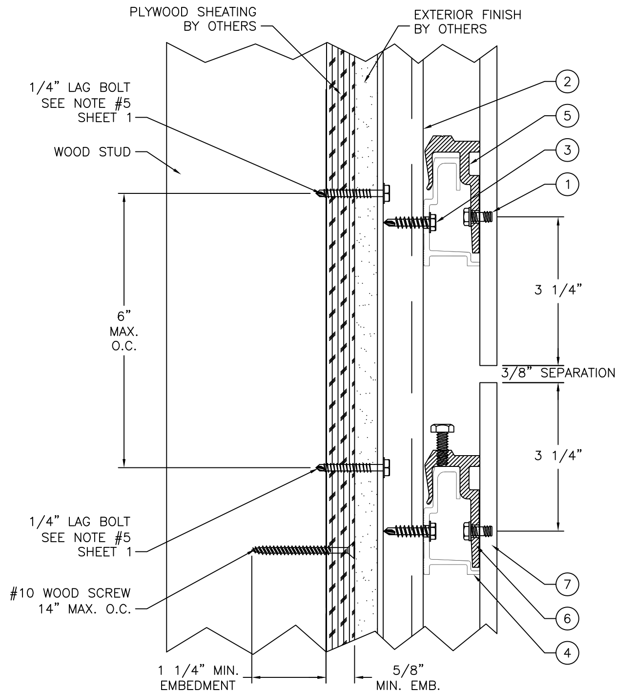
SECTION B-B INSTALLATION DETAIL 5/8" PLYWOOD SHEATHING (WOOD FRAMING)
