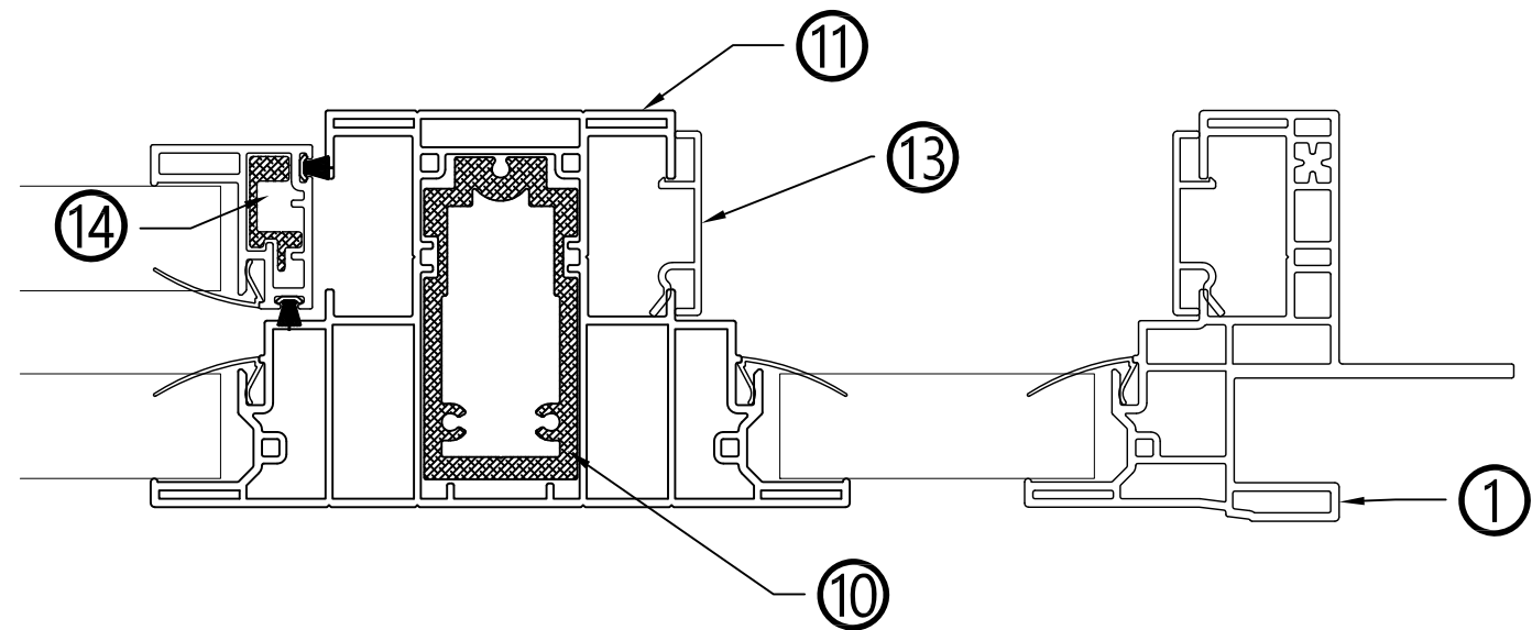
TYP. HORIZ. SECTION SH|SSPW MULLION
