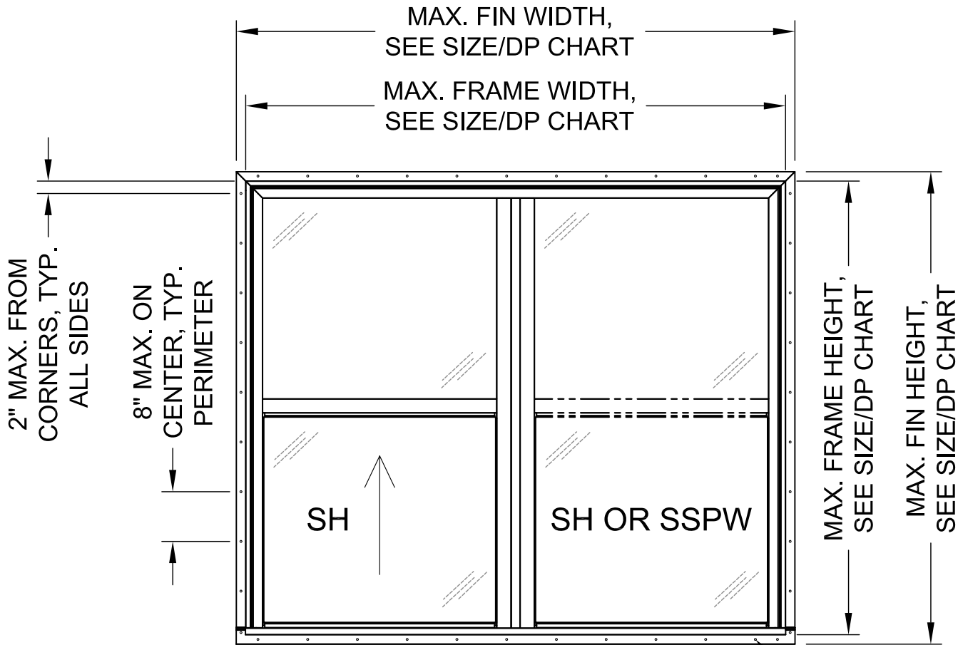
ELEVATION - FIN INSTALLATION
