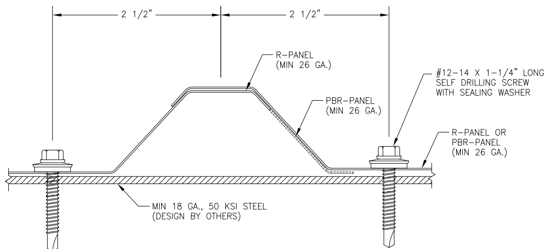
DETAIL 1
