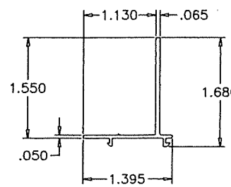
(E5) NAIL FIN ADAPTER
