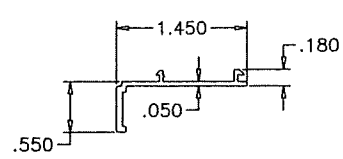
(E6) FLANGE ADAPTOR
