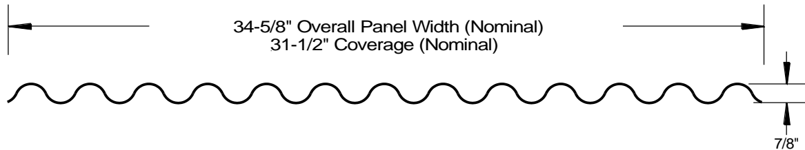
Typical Panel Profile View
