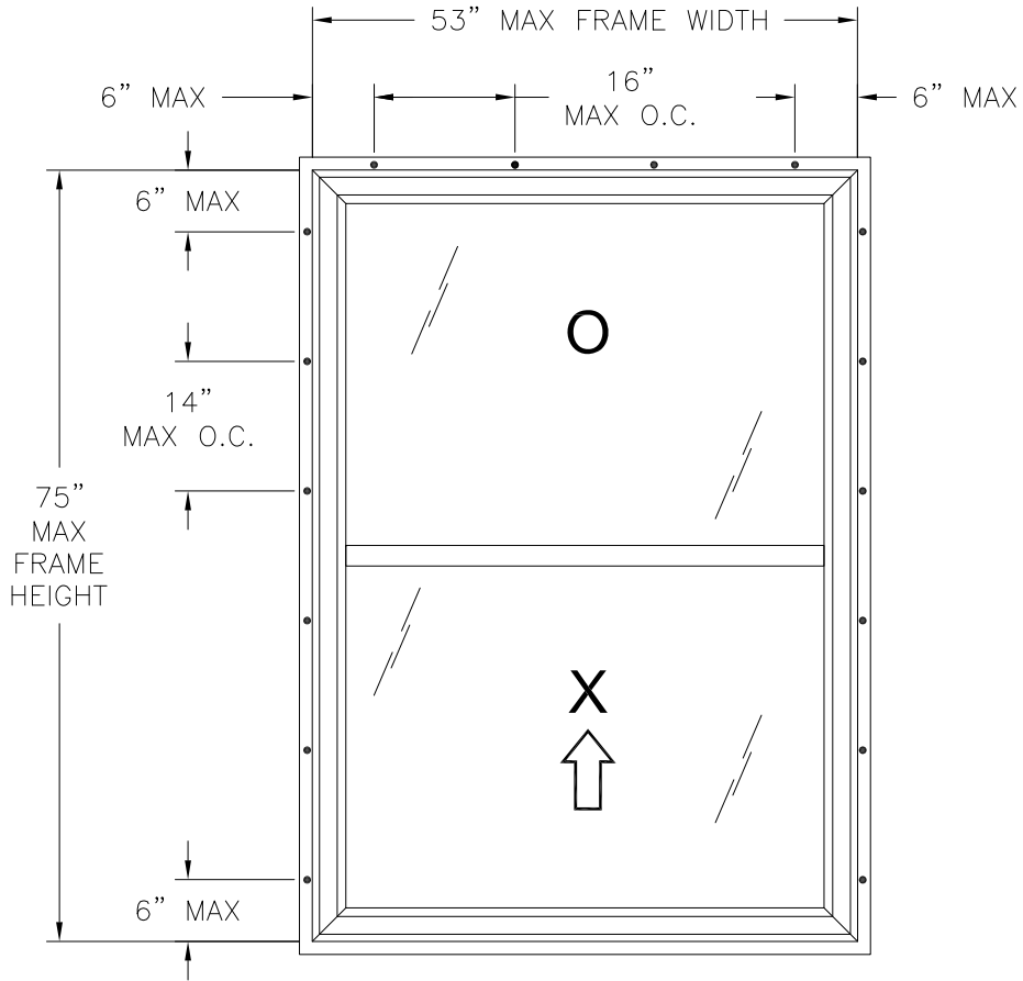
SHORELINE SINGLE HUNG WINDOW EXTERIOR VIEW FIN INSTALLATION
