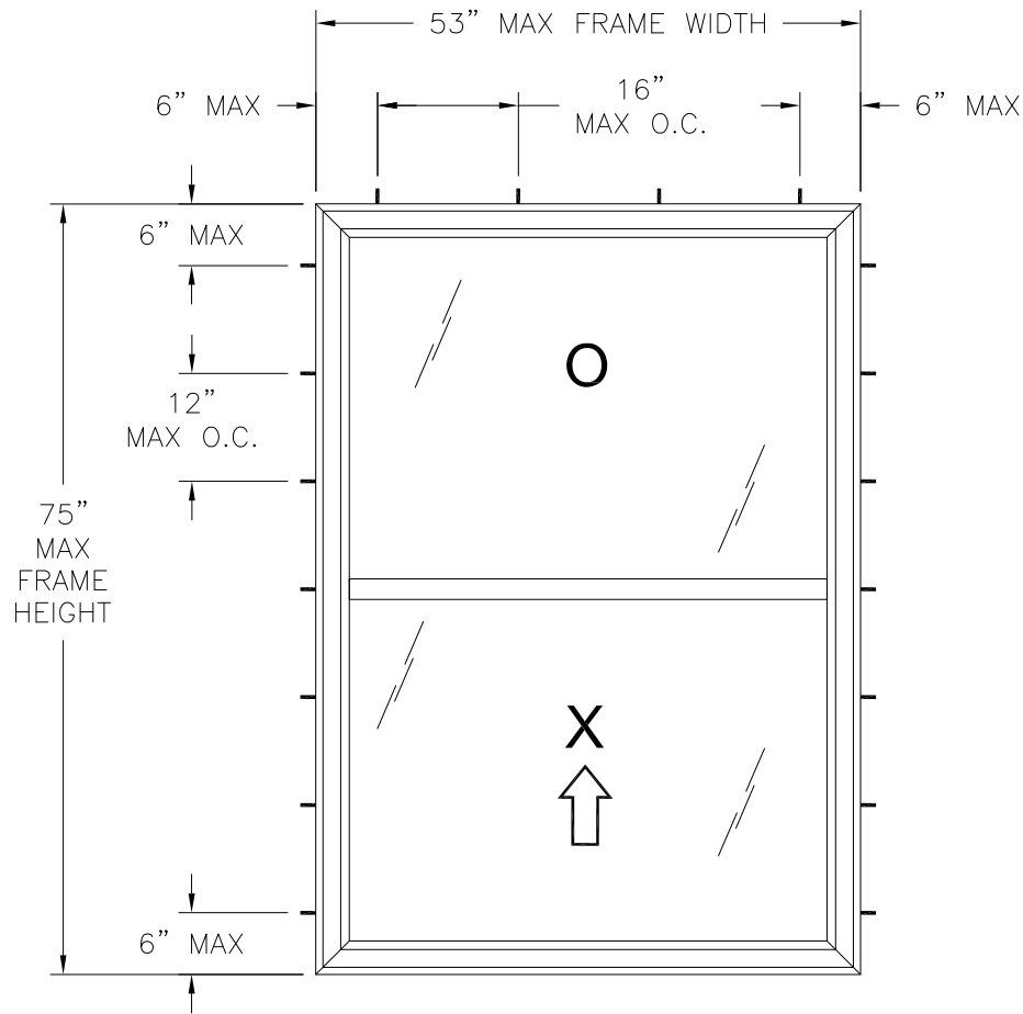
SHORELINE SINGLE HUNG WINDOW EXTERIOR VIEW FRAME FLUSH INSTALLATION
