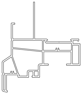
4252 FRAME (OPTIONAL) FIN INSTALLATION
