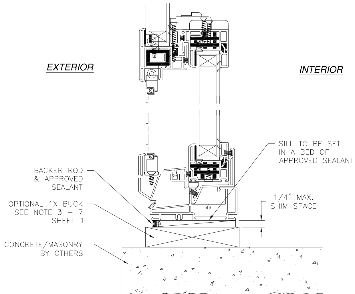
VERTICAL CROSS SECTION CONCRETE/MASONRY INSTALLATION HEAD AND SILL SHOWN, JAMBS SIMILAR
