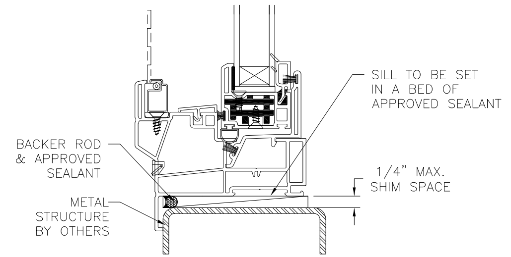
VERTICAL CROSS SECTION METAL STRUCTURE INSTALLATION HEAD AND SILL SHOWN, JAMBS SIMILAR
