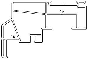
4252 FRAME (OPTIONAL) FLUSH INSTALLATION
