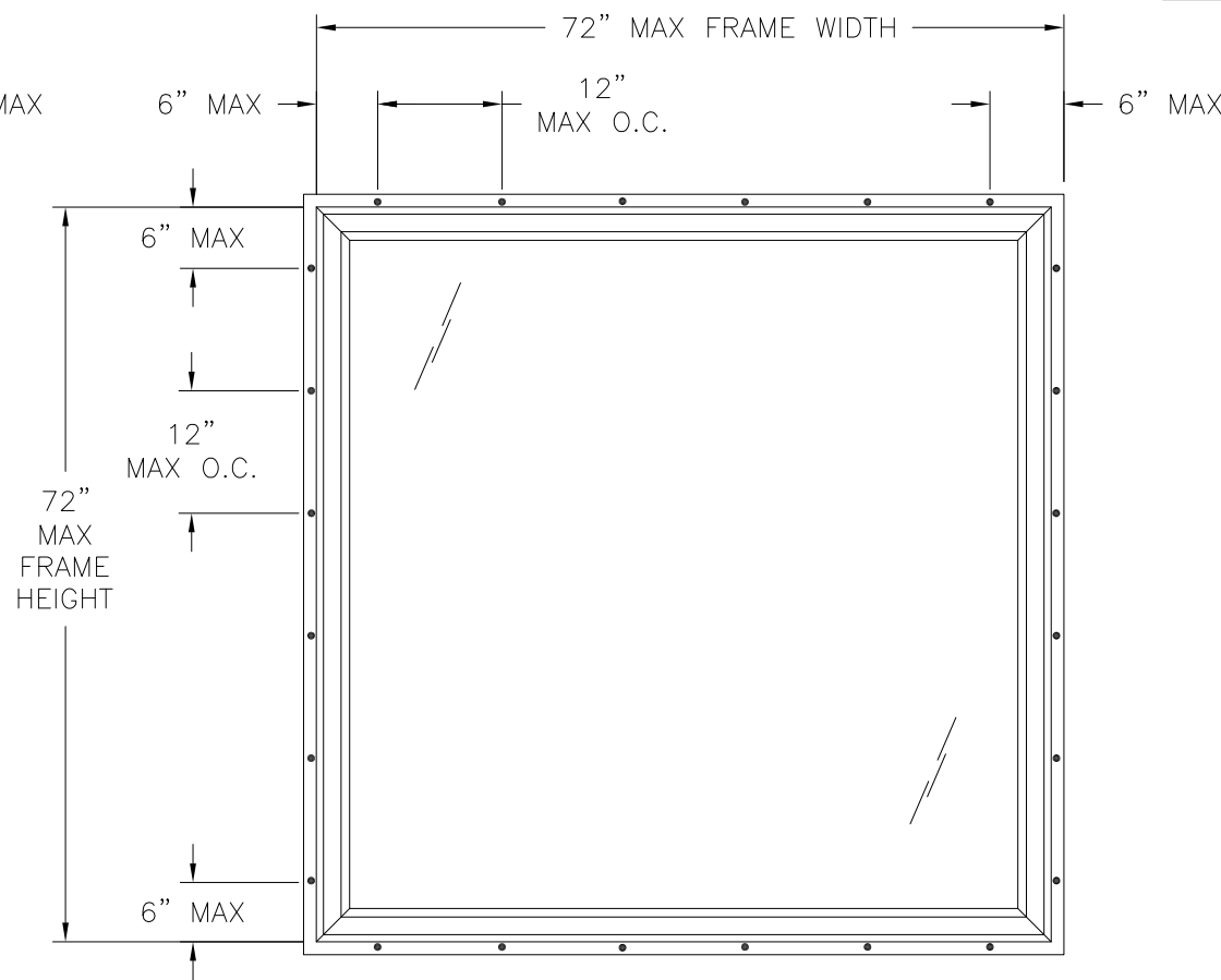
SHORELINE SL 3100 PW 7272 EXTERIOR VIEW FIN INSTALLATION
