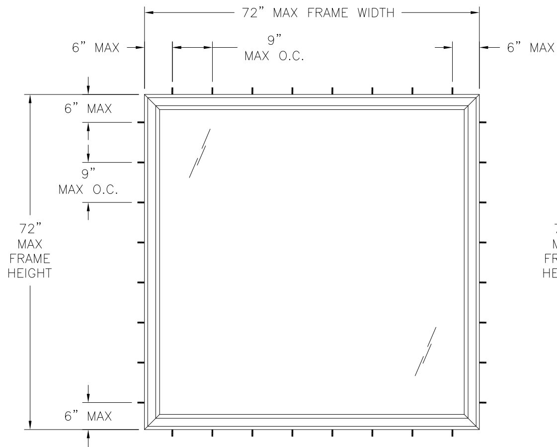
SHORELINE SL 3100 PW 7272 EXTERIOR VIEW FRAME FLUSH INSTALLATION
